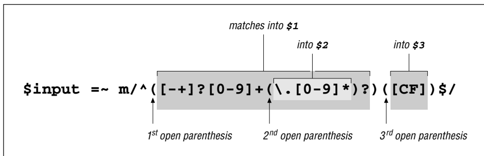
Figure 2-3: Nesting parentheses
